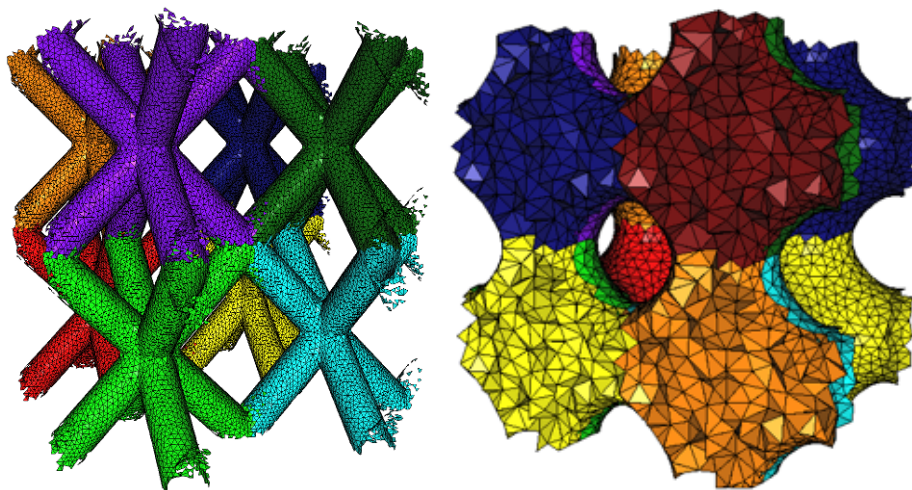
FIGURE 5 – Periodic surface (left) and volume (right) meshes. (left) Data courtesy of Maarten Moesen, Department of Metallurgy and Materials Engineering (MTM), K.U. Leuven, Belgium.
