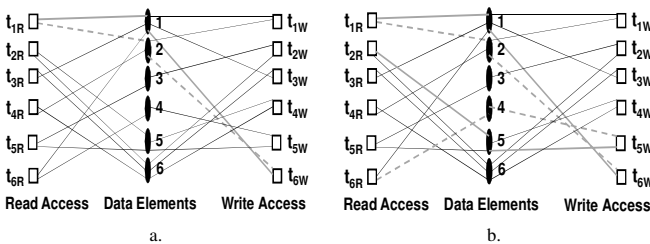
Figure 7: Conflict Free Edge Coloring of Par_1
