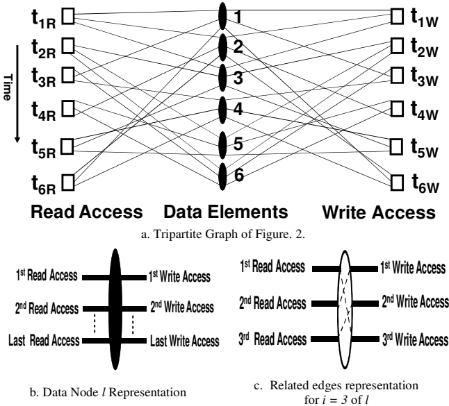
Figure 3: Tripartite Graph Representation
