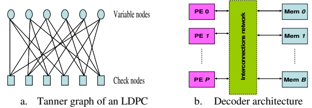
Figure 1: LDPC code and decoder architecture
