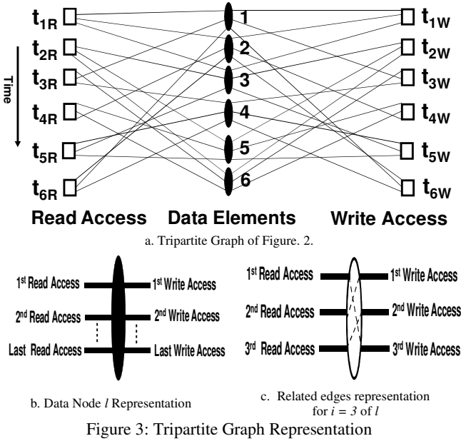
Figure 3: Tripartite Graph Representation
