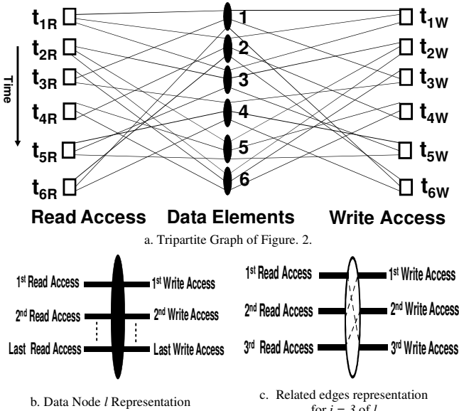
Figure 3: Tripartite Graph Representation
