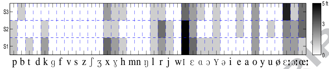
Figure 5: Contribution of phoneme states at the optimal number of features. S_i is the i -th state of a phoneme.
