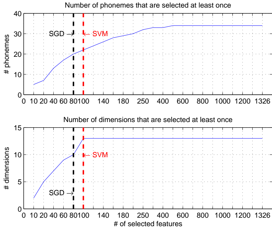
Figure 6: The number of phonemes (top) and dimensions (bottom) that are selected at least once as a function of the size of the reduced feature set
