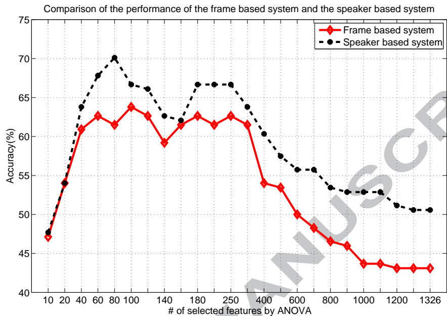
Figure 10: Identification accuracy of the speaker based versus the frame based SGD system as a function of the size of reduced feature set dimension.
