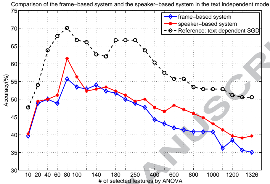
Figure 11: Identification accuracy of the speaker based versus a frame based SGD system as a function of the reduced feature set dimension in the text independent case.
