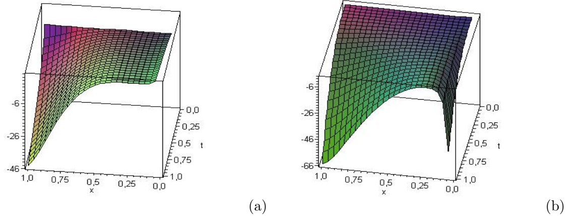
Figure 3: The numerical solutions of u(x, t) : (a) \alpha = 1 et \beta = 1.2 , (b): \alpha = 0.75 et \beta = 1.75 .
