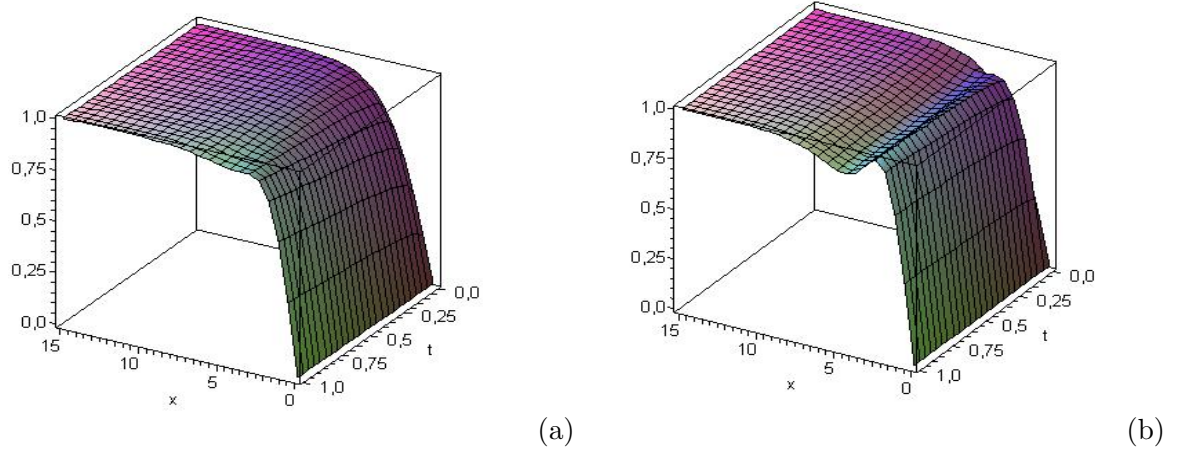
Figure 2: The numerical solutions of u(x, t) : (a) \alpha = 0.50 (b) \alpha = 0.05 .
