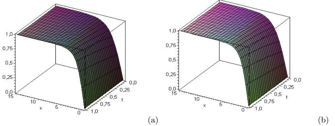
Figure 1: The numerical solutions of u(x, t) : (a) by ADM (20) and (b) the exact solutions given in (15).
