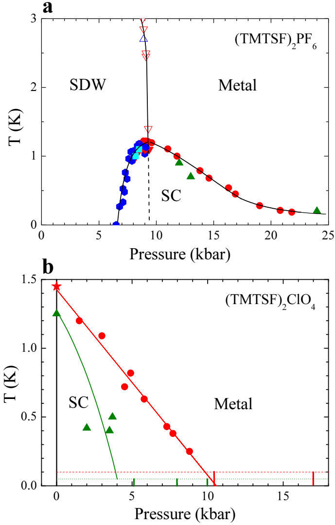
FIG. 1: (a) (P - T) phase diagram of (\text{TMTSF})_2\text{PF}_6 deduced from resistivity measurements. The data points below 9.4 kbar (the coexistence regime) are deduced from measurements along the three crystallographic axes: down triangles for \rho_a , squares for \rho_b , hexagons for \rho_c , empty symbols for T_{SDW} and full symbols for T_{SC} [22, 23]. Above the critical pressure (9.4 kbar), only longitudinal resistivity data are plotted: (red) circles from this work and (green) triangles from Ref.[24]. (b) Pressure dependence of the superconducting transition of (\text{TMTSF})_2\text{ClO}_4 deduced from longitudinal resistivity measurements: (red) circles from this work (the star at 1 bar is derived from a \rho_c measurement[25]) and (green) triangles from Ref.[9]. Dashed-dotted horizontal lines (red or green) indicate the lowest reached temperature without superconductivity for both studies. The (red) continuous line is a linear fit of the data including the point at 1 bar.
