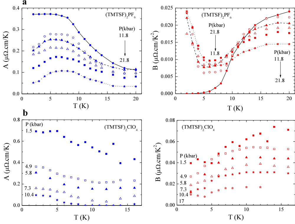
FIG. 5: Temperature dependence of A (left) and B (right) coefficients of the polynomial fit, \rho(T) = \rho_0 + AT + BT^2 at different pressures for (\text{TMTSF})_2\text{PF}_6 (a) and (\text{TMTSF})_2\text{ClO}_4 (b). Each temperature point corresponds to the center of a 4K window used for the fit. As far as (\text{TMTSF})_2\text{PF}_6 is concerned, this figure shows that under 11.8 kbar B is zero and A constant below 4 K within the accuracy of the measurements and data processing. However, a small low temperature quadratic term arises at larger pressures, (see Fig.7).
