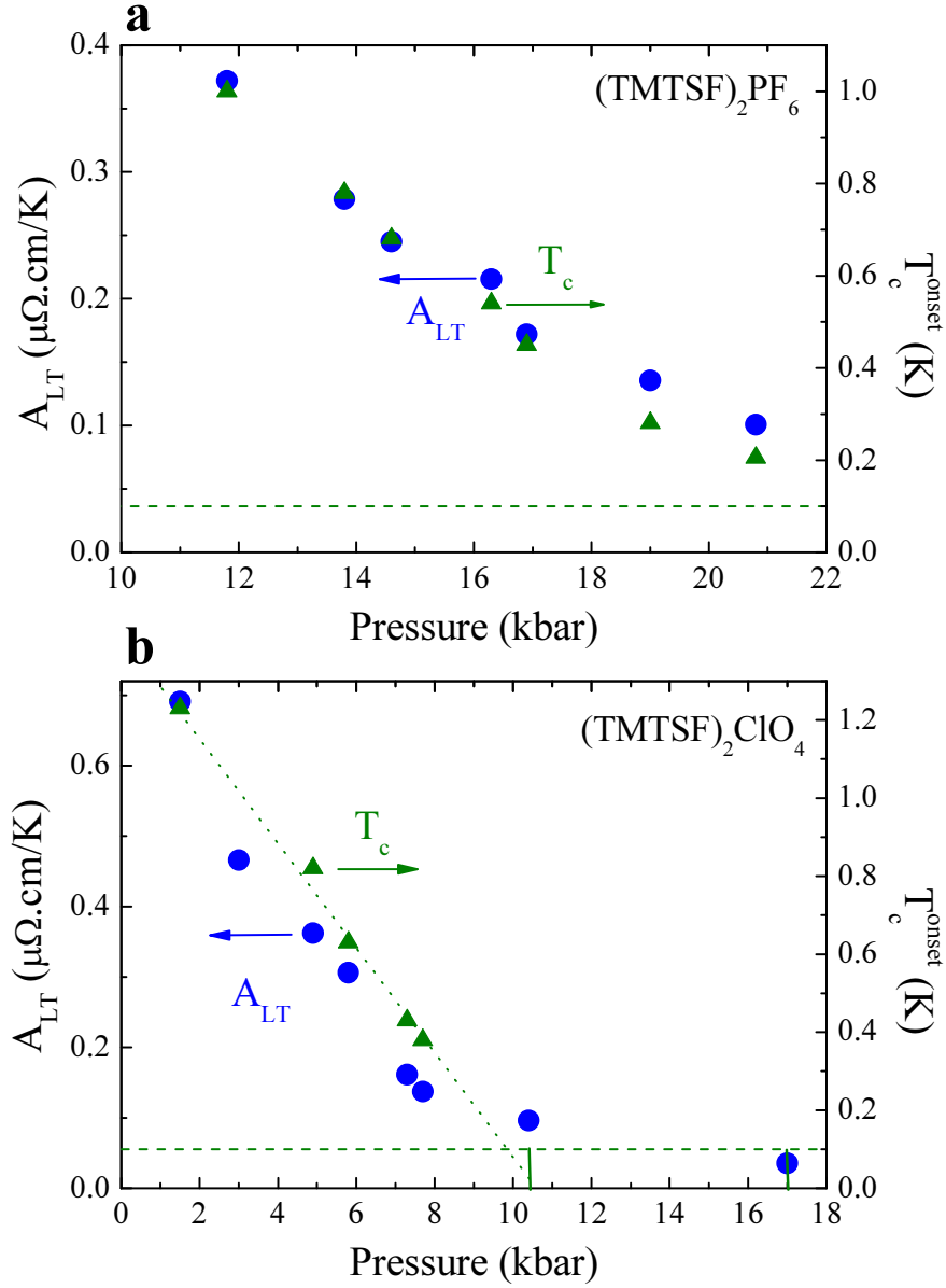
FIG. 6: Pressure dependence of T_c^{\text{onset}} and A_{LT} coefficient for (\text{TMTSF})_2\text{PF}_6 (a) and (\text{TMTSF})_2\text{ClO}_4 (b). A_{LT} is obtained from the second order polynomial fit described in the text in the temperature window corresponding to its maximum value for (\text{TMTSF})_2\text{PF}_6 and in the 0.1 – 4 K window for (\text{TMTSF})_2\text{ClO}_4 . The horizontal dashed lines indicate our lowest reached temperature, 0.1K. For (\text{TMTSF})_2\text{ClO}_4 , the vertical lines below this temperature indicate the pressure points at 10.4 and 17kbar without superconductivity and the dotted line is a linear fit of T_c^{\text{onset}} data points.
