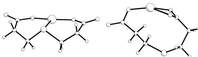
Fig. 2. Optimised structures of models I-II .
