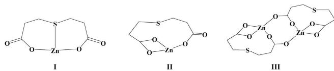
Scheme 1. Models of [\text{Zn}(\text{tdp})] theoretically studied.
