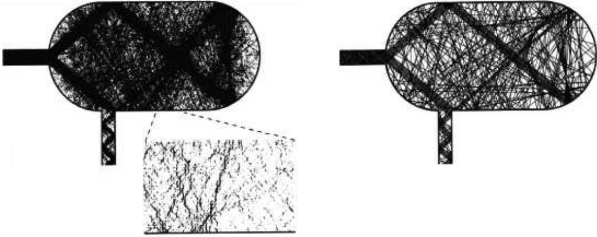
FIGURE 16. Left: density plot of a scattering state |u_E(x)|^2 , with incoming part u_{E,in} a plane wave in the left lead into the stadium-shaped cavity. Right: corresponding classical trajectories incoming from the left opening with angles \pm\theta_n . Reprinted with permission from H. Ishio and J.P. Keating, J. Phys. A 37 (2004) L217–L223. Copyright 2004 by the Institute of Physics.
