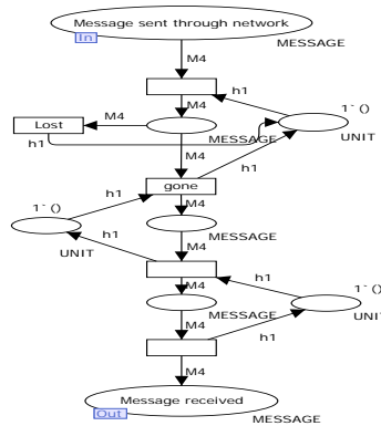
Figure 5. Network model
