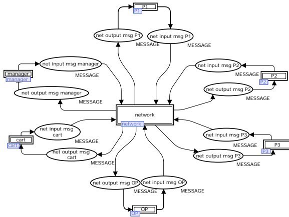
Figure 4. Global cooperation model
