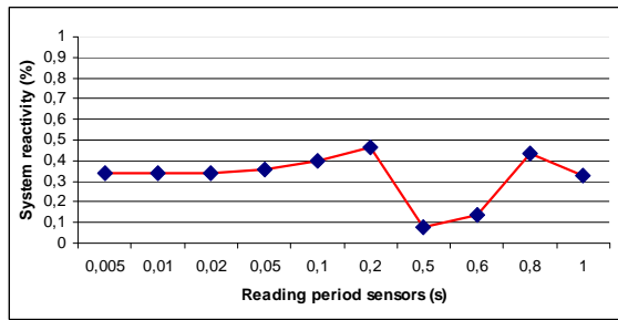
Figure 9. Influence of the reading period sensors on the system reactivity
