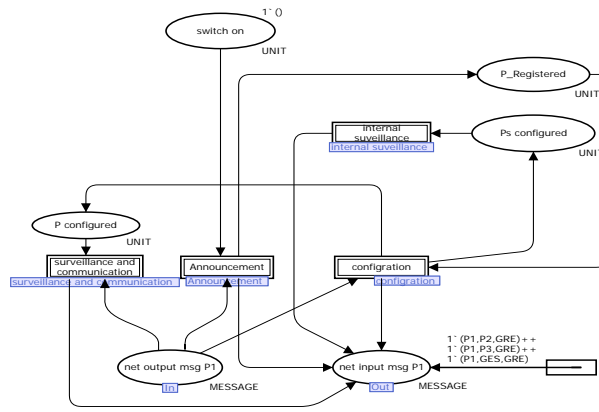
Figure 6. Intelligent product model
