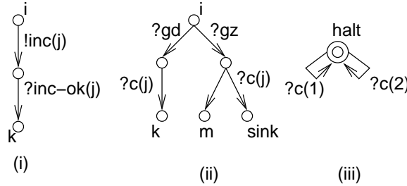
Figure 7: Transitions of process A
