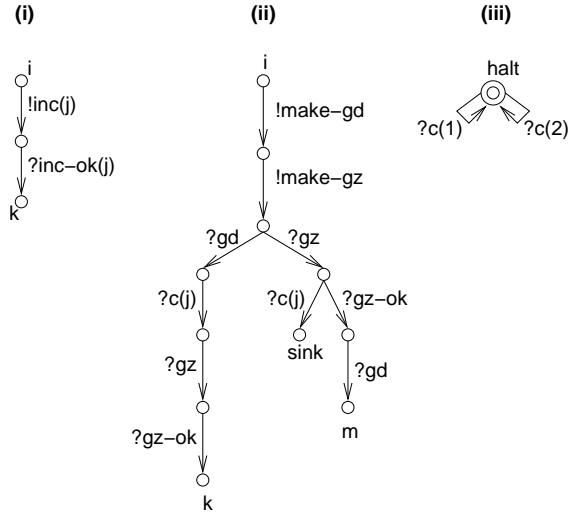
Figure 10: Transitions of process A in Phase (ii)
