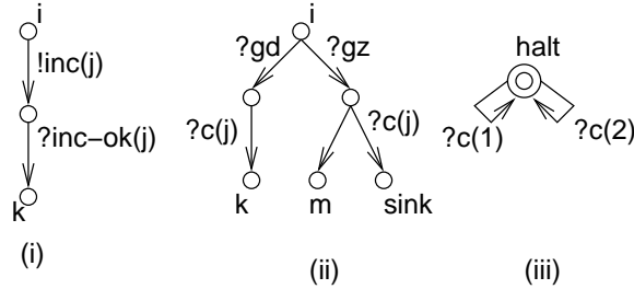
Figure 7: Transitions of process A
