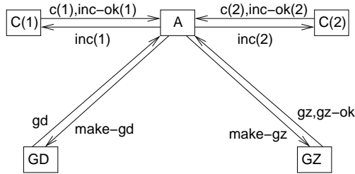
Figure 8: The architecture of \mathcal{A} in Phase (ii)
