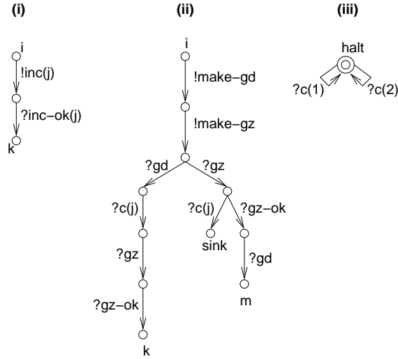
Figure 10: Transitions of process A in Phase (ii)
