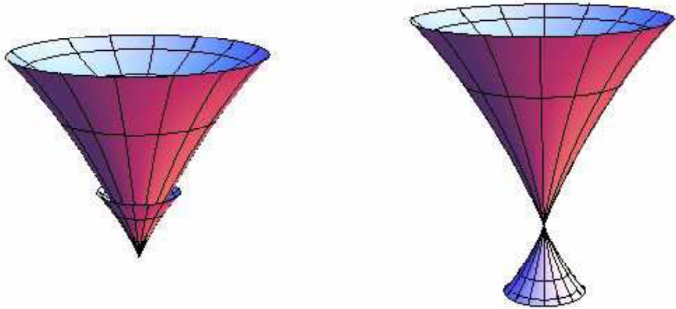
Figure 6. Noncongruent hedgehogs with the same curvature function
