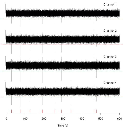
Figure 1: Detection of LFP activity on the first time-derivative of the data. The same scale applies to all channels (vertical bar: 200 \mu\text{V} / \text{ms} ). Channel specific detection threshold shown in dashed red. Detected events are shown as vertical red bar at bottom.
