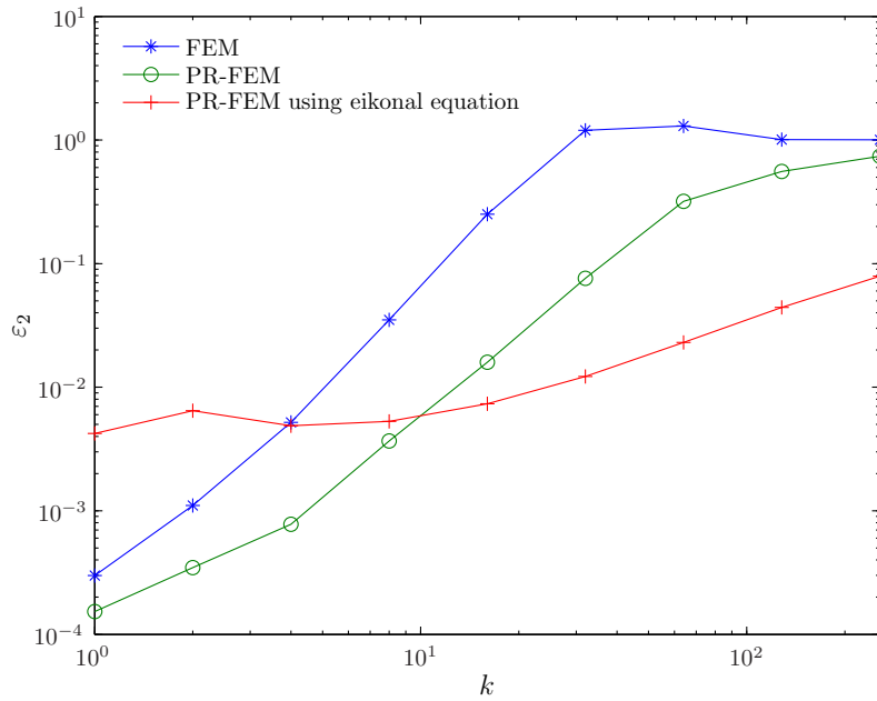
Fig. 20. Dirichlet problem: Evolution of the error \varepsilon_2 with respect to the wavenumber k ( k = 1 to k = 256 ) using a fixed uniform mesh of 7592 triangles. The results are presented for the classical FEM, the PR-FEM with the low-order propagator and the eikonal equation.
