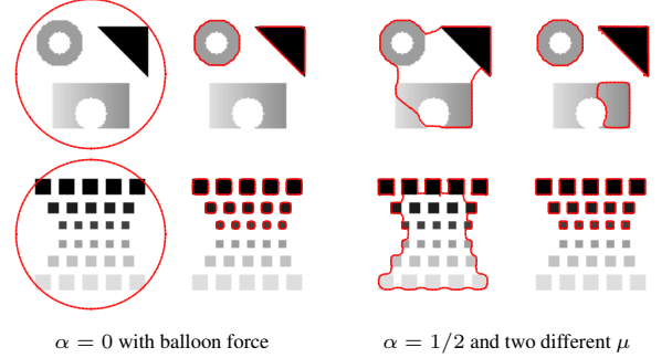
Fig. 2. Final curves of models given in (8): \alpha = 0 with balloon force term (GAC), \alpha = 1/2 (IAC) with two different but close parameters \mu . GAC: \mu = 1, \eta = -0.3 . IAC: (top) \mu = 3.6 and 3.5 , (bottom) \mu = 1 and 0.9 . IAC used initial curves given in Fig. 1.
