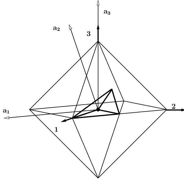
Figure 7: The unit vectors 1, 2, 3, the Weyl vectors a_1, a_2, a_3 of the Coxeter group \Gamma = \circ - \circ - \circ - \circ , and the Coxeter simplex bounded by the Weyl reflection planes. 48 Coxeter simplices share a vertex and form the octahedral manifolds N_4, N_5, N_6 .
