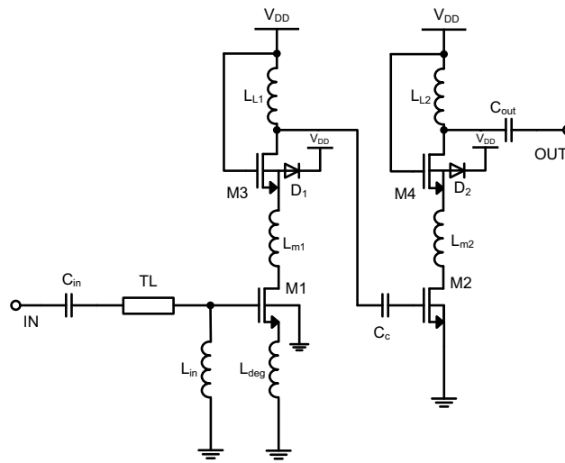
Fig. 2. Circuit schematic of the employed LNA [13]
