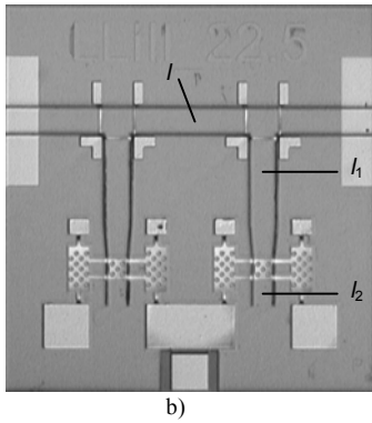
Fig. 14. Fabricated 60-GHz loaded line phase shifter. Electrical schematic (a) and microphotograph (b).
