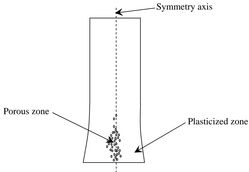
Figure 2. Schematic of the cylinder profile and porosity contour after the impact
