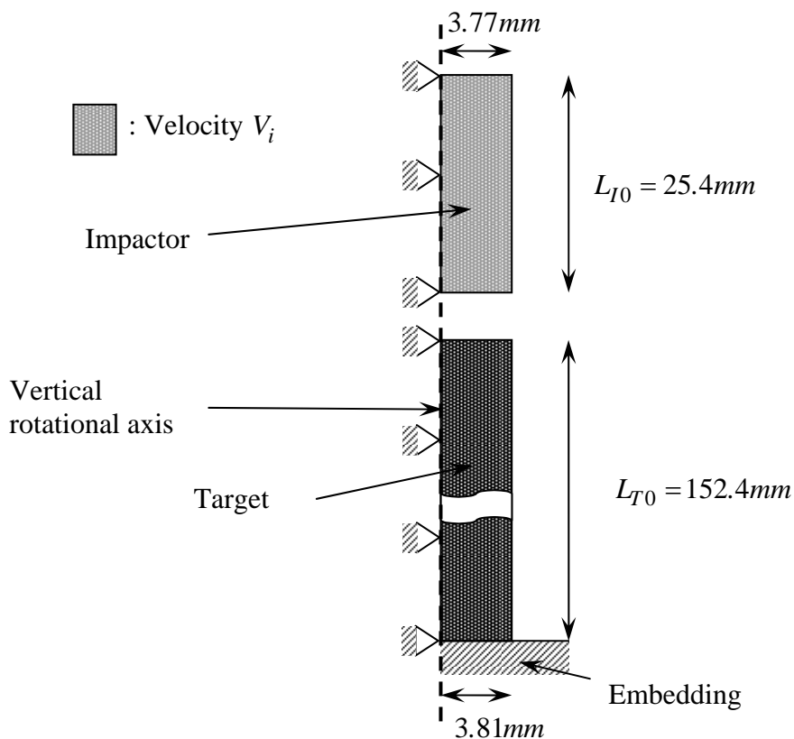
Figure 3. Schematic of the target and impactor for Taylor impact test (Rod-on-Rod).
