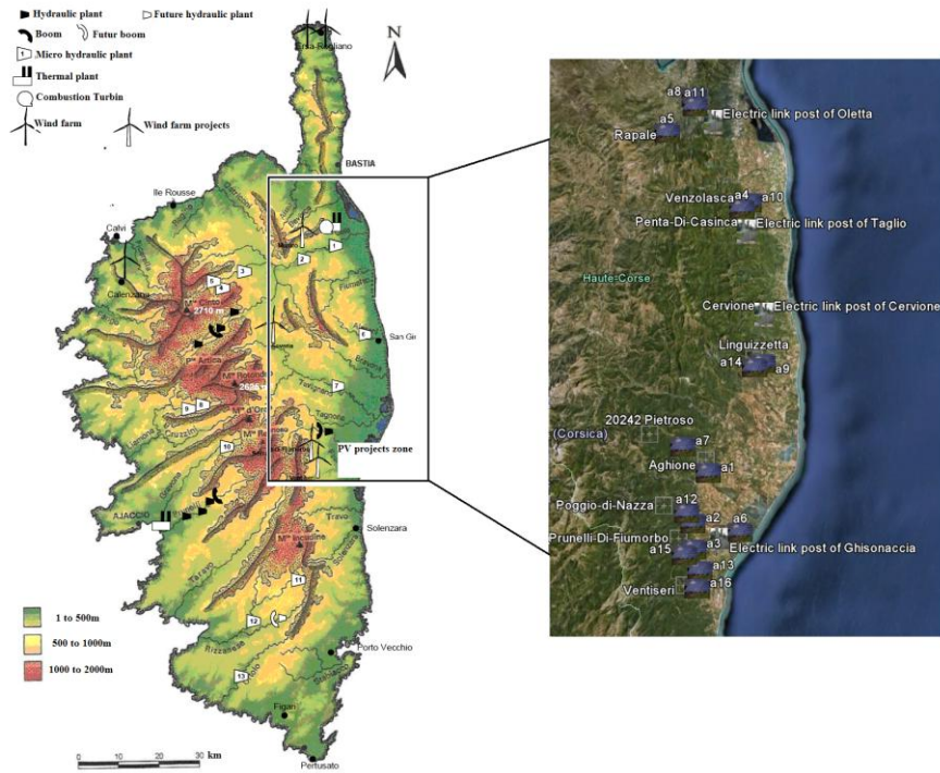
3 Figure 2: Geographic location of electricity production means in Corsica and areas concerned by 4 photovoltaic plants.
