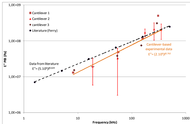
Fig. 2. Frequency-dependent loss modulus of PIB (log-scale).
