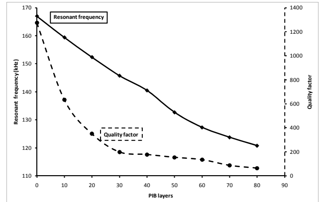
Fig. 1. Evolution of both the resonant frequency and total quality factor after successive PIB layers depositions (third flexural mode of cantilever 1).
