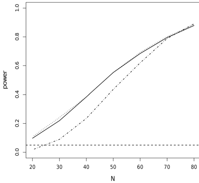
Figure 1. Power of the sampled posterior ( p_{sp} ; solid line), half-sample ML ( p_{MLs} ; dotted line) and posterior predictive ( p_{pop} ; dotted-dashed line) p-values. Power of the p-values p_{sp} (solid line), p_{MLs} (dotted line) and p_{pop} (dotted-dashed line) used with the maximum test statistic to detect departures from the Poisson distribution at the level of p=0.05 when data are distributed according to a Polya distribution with n_{max}=5 . Power is plotted as a function of sample size N varying between 20 and 80. p_{sp} and p_{MLs} were equivalent in terms of power, and both were more powerful than p_{pop} except at the highest sample sizes. The dotted baseline level corresponds to p=0.05 . doi:10.1371/journal.pone.0014770.g001
