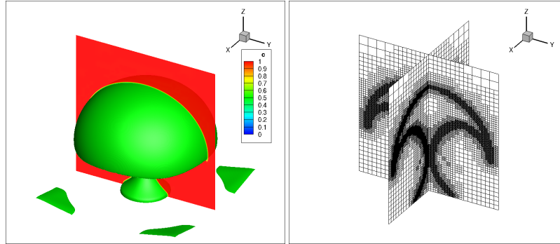
Fig. 3 3D premixed flame interacting with a toroidal vortex. Solution of variable c at t_* = 1.1 \times 10^{-3} showing isosurface c = 0.5 (left) and corresponding adapted mesh (right). Finest grid: 256^3
