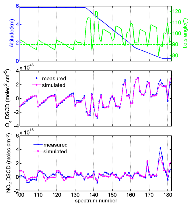
Fig. 8. DSCD measurements during the as0831 flight (8 April 2008). The upper panel shows the plane altitude (blue) and the telescope line-of-sight angle (green, 0° is nadir, 90° horizontal). On the middle and bottom panels, measured DSCD, respectively of O 4 and NO 2 , are compared with simulations. Oscillations on the DSCD series are caused by the telescope scanning. Discrepancies between measured and simulated DSCD are larger in the boundary layer, where true aerosol extinction and NO 2 concentration are different from the model.
