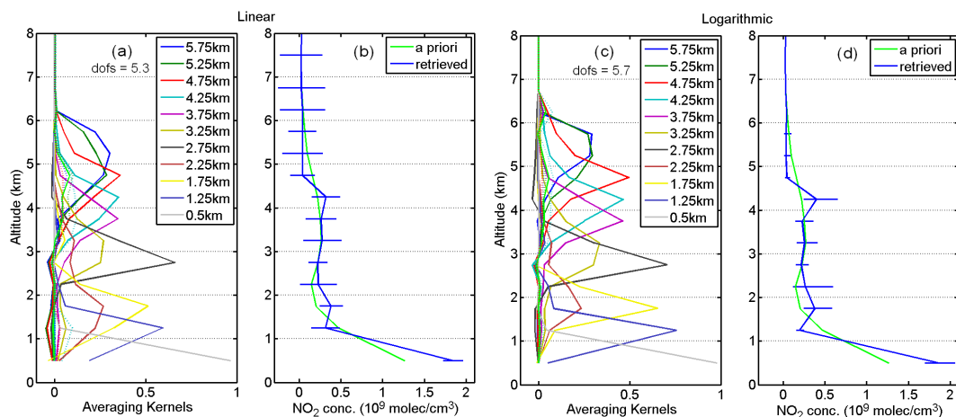
Fig. 11. Comparison of the NO 2 profile retrieval using linear (left) and logarithmic (right) weighting functions for the sounding of the as0831 flight (8 April 2008). The two panels show the respective averaging kernels and retrieved profiles. The results are very close, contrary to the aerosol extinction retrieval.
