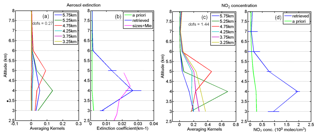
Fig. 12. Retrieved extinction and NO 2 profiles for the sounding of the as0833 flight (9 April 2008). Under 3 km high, the radiative transfer is too strongly affected by clouds to enable quantitative retrievals. Around 4 km high, an enhanced layer is measured for both extinction and NO 2 .
