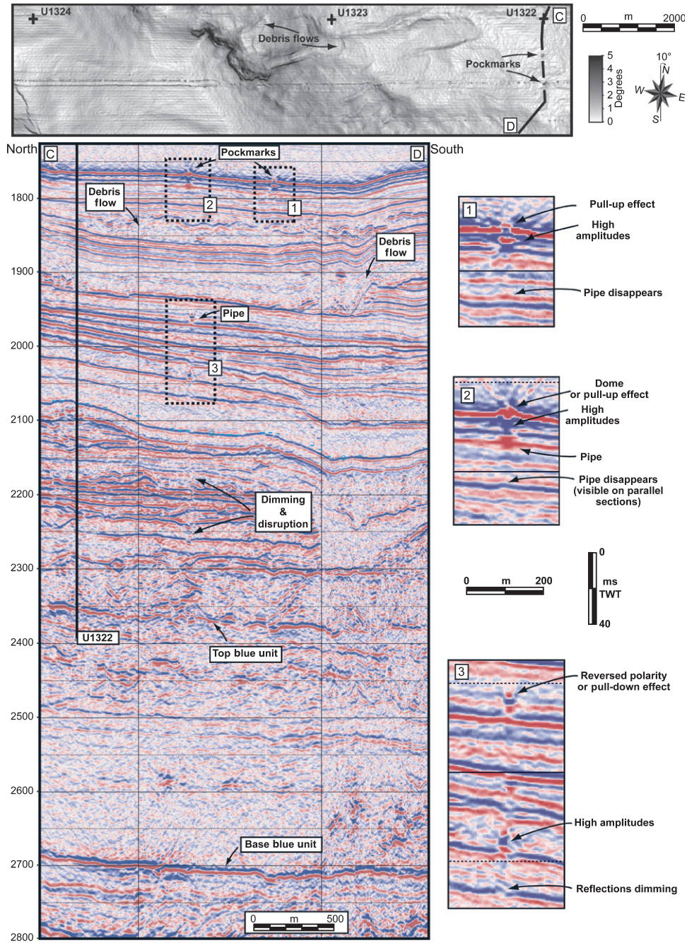
Fig. 4. Top: Dip map of seafloor from high resolution (6.25 × 6.25 m) 3D seismic data. Pockmarks are only identified on these high resolution data, and not on conventional 3D seismic data. Bottom: Seismic profile CD (see Fig. 1 for location), extracted from high resolution (6.25 × 6.25 m) 3D seismic data, crossing a pockmark and its related underlying pipe (see zoomed in views 1–3 for details). Even if its identification is tenuous, the pipe seems to penetrate the Blue Unit. Most of the pipes in the area source from the Blue Unit or from shallower depths, but most of the pockmarks are concentrated at the toe of the slope, close to Site U1322 and to the key-well 899-1. They have been formed during exploration drilling operations prior to IODP Expedition 308 drilling, and Shell’s personal communication).
