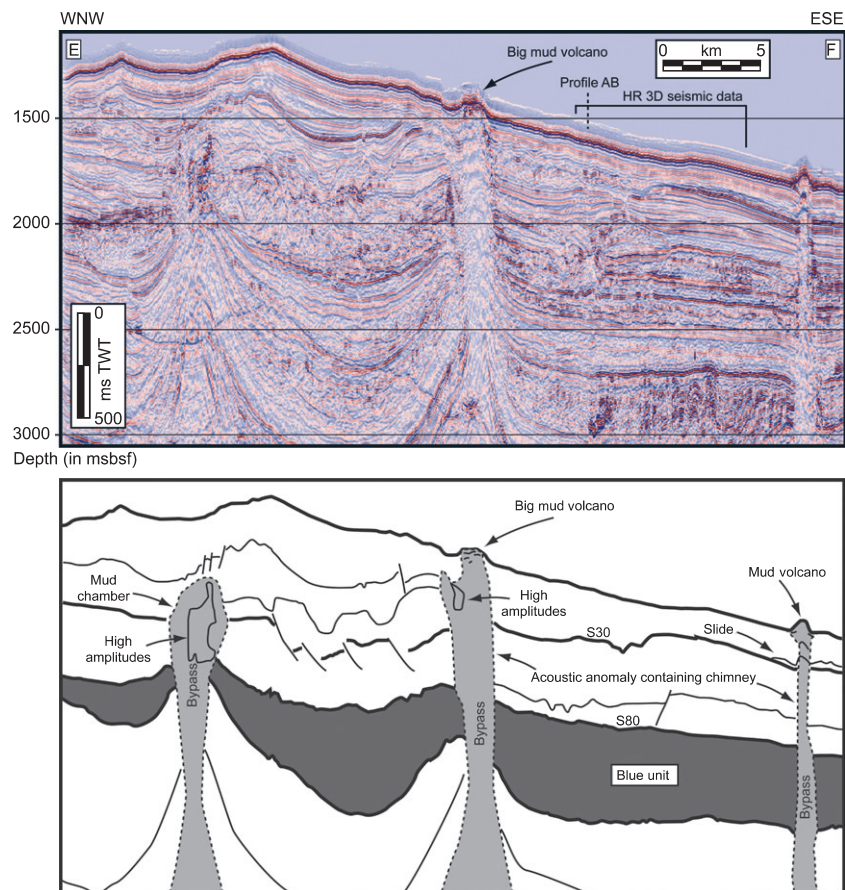
Fig. 5. Seismic profile EF (see Fig. 1 for location), extracted from conventional ( 12.5 \times 12.5 m) 3D seismic data, showing mud volcanoes and piercing mud structures. The underlying conduits are as large as the mud volcanoes themselves, ranging from 500 to 2000 m in diameter. All mud volcanoes identified in the study area have a conduit that penetrates deeper than the Blue Unit, suggesting that the fluid overpressure from below the Blue Unit is released through these conduits and bypass the upper sequence over the Blue Unit.
