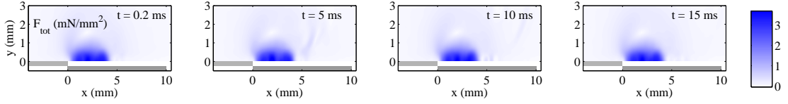
Figure 11. Instantaneous total force field obtained using the gradient method ( 12kV_{pp} , 2kHz ).
