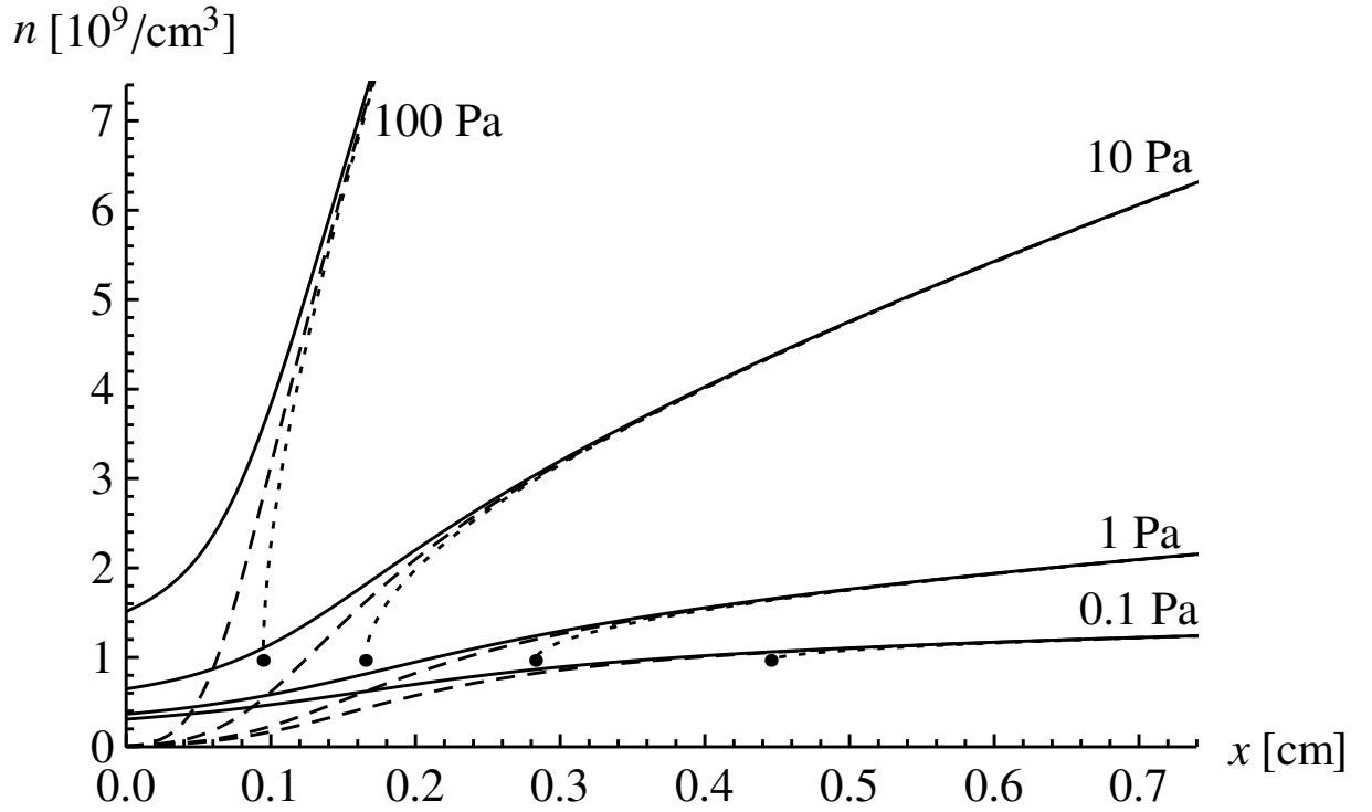
FIG. 1: Densities of the electrons (thin) and ions (thick) in an argon sheath facing a floating wall, for an electron temperature T_e = 3\text{ eV} and an ion current j_i = 0.04\text{ mA/cm}^2 . The neutral gas pressure values are 0.1 Pa, 1 Pa, 10 Pa, and 100 Pa; corresponding to a nominal scale ratio \lambda_D/\lambda of 0.01, 0.1, 1, and 10, respectively. Dashed are the plasma solutions which end in a singularity at the conventional Bohm point v_B = \sqrt{T_e/m_i} = 2700\text{ m/s} and n_B = 9.7 \times 10^8\text{ cm}^{-3} .
