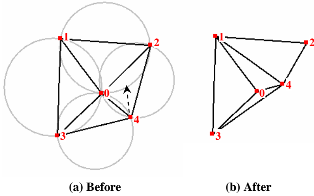
Figure 1. (a) Delaunay triangulation (b) Flip operation resulting from node 4's movement
