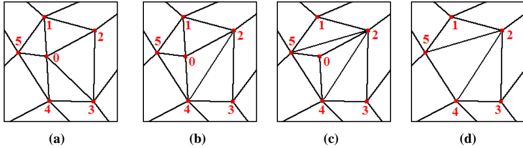
Fig. 8 Deletion of node 0
