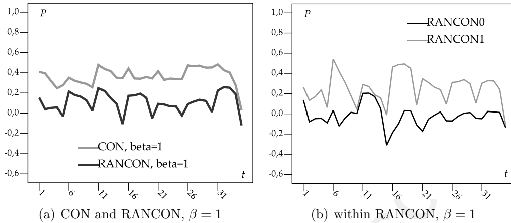
Figure 3: Evolution of average degree of price collusion in RANCON, \beta = 1
