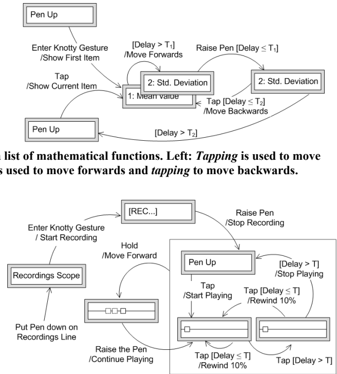
Figure 8. Recording and replaying an audio clip: state transitions and corresponding screens.
