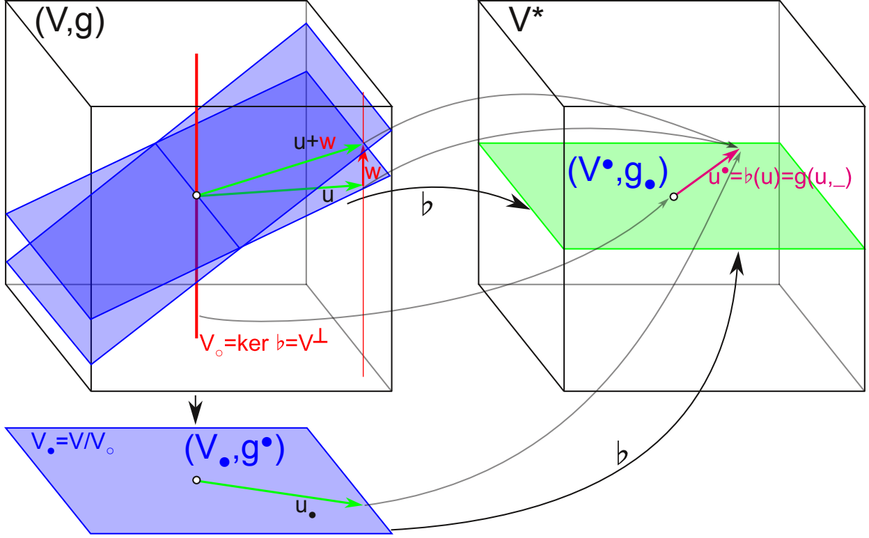
FIGURE 1. (V, g) is an inner product vector space. The morphism b : V \rightarrow V^* is defined by u \mapsto u^\bullet := b(u) = u^b = g(u, \_) . The radical V_\circ := \ker b = V^\perp is the set of isotropic vectors in V . V^\bullet := \text{im } b \leq V^* is the image of b . The inner product g induces on V^\bullet an inner product defined by g_\bullet(u_1^b, u_2^b) := g(u_1, u_2) , which is the inverse of g iff \det g \neq 0 . The quotient V_\bullet := V/V_\circ consists in the equivalence classes of the form u + V_\circ . On V_\bullet , g induces an inner product g^\bullet(u_1 + V_\circ, u_2 + V_\circ) := g(u_1, u_2) .
