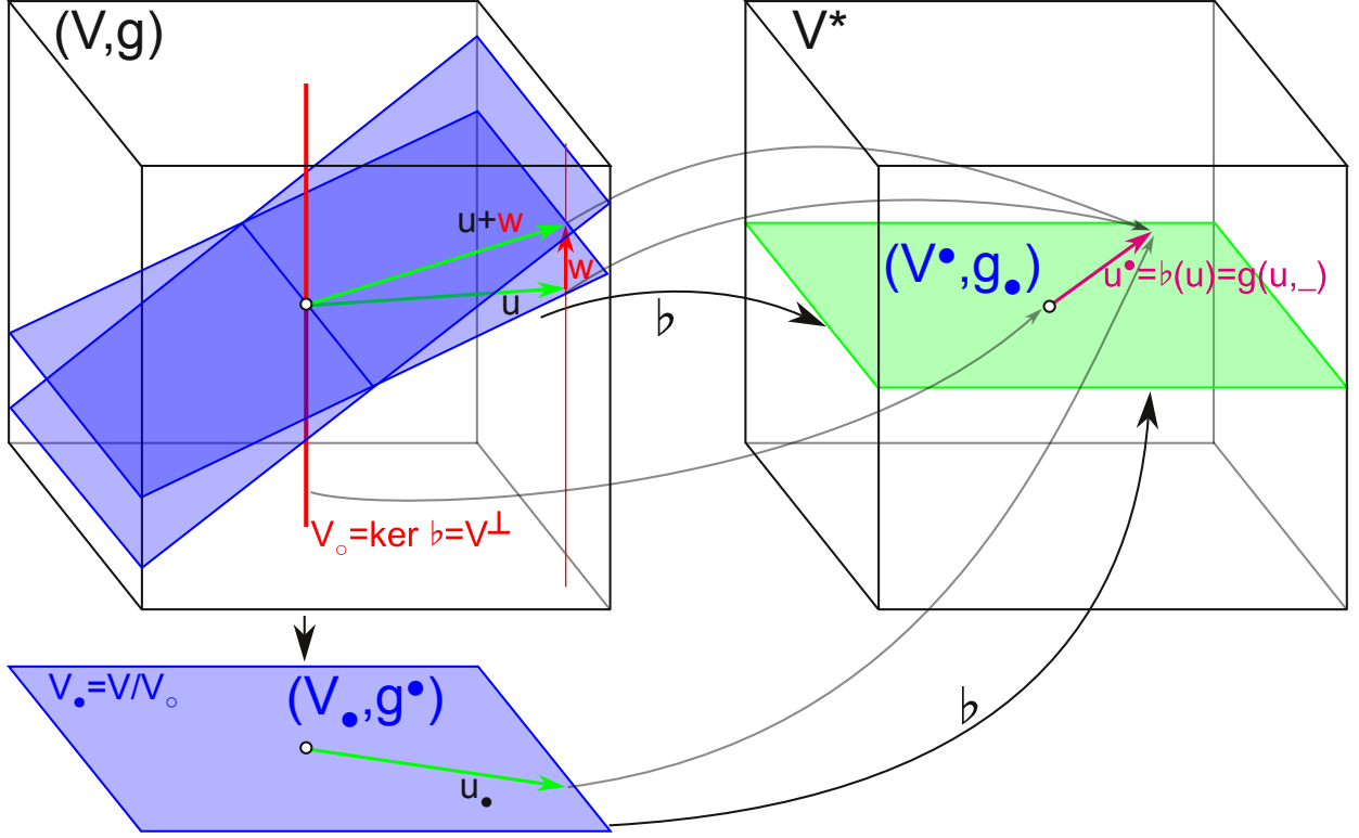
FIGURE 1. (V, g) is an inner product vector space. The morphism b : V \rightarrow V^* is defined by u \mapsto u^\bullet := b(u) = u^\flat = g(u, \_) . The radical V_\circ := \ker b = V^\perp is the set of isotropic vectors in V . V^\bullet := \text{im } b \leq V^* is the image of b . The inner product g induces on V^\bullet an inner product defined by g_\bullet(u_1^\flat, u_2^\flat) := g(u_1, u_2) , which is the inverse of g iff \det g \neq 0 . The quotient V_\bullet := V/V_\circ consists in the equivalence classes of the form u + V_\circ . On V_\bullet , g induces an inner product g^\bullet(u_1 + V_\circ, u_2 + V_\circ) := g(u_1, u_2) .
