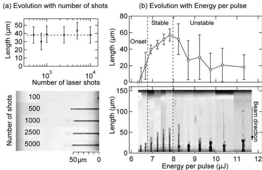
Fig. 2 (a) Evolution of channel length (top) and morphology (bottom) with number of laser shots at 7 \mu\text{J}/\text{pulse} , 100Hz.
