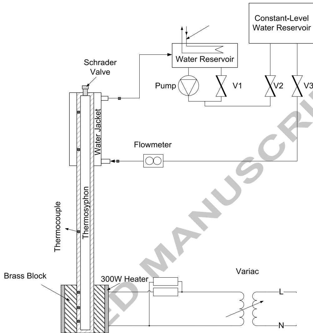
Figure 2: Schematic diagram of thermosyphon test rig
