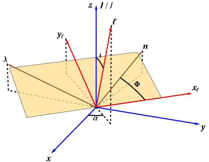
FIG. 1: We show (i) the source frame defined by the orthonormal basis (\mathbf{x}, \mathbf{y}, \mathbf{z}) , (ii) the instantaneous orbital plane which is described by the orthonormal basis (\mathbf{x}_\ell, \mathbf{y}_\ell, \boldsymbol{\ell}) , (iii) the moving triad (\mathbf{n}, \boldsymbol{\lambda}, \boldsymbol{\ell}) , and (iv) the direction of the total angular momentum \mathbf{J} (agreeing by definition with the z -direction). Dashed lines show projections into the x - y plane.
