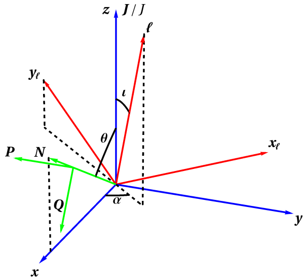
FIG. 2: Similar as Fig. 1 but with the direction of the source \mathbf{N} indicated together with a choice of convention for the two polarization vectors \mathbf{P} and \mathbf{Q} .
