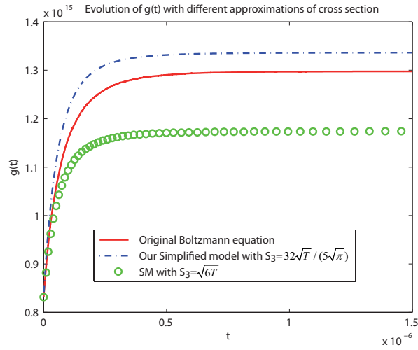
FIGURE 3. Evolution of g(t) with a = 0 , \gamma = 0.6 . Hard Spheres. In that case ( a = 0 ), only the growing part of g(t) is represented (65). We tested our simplified model versus the original Boltzmann one with two different approximations of the cross section. The formula (28) fits the best with the original Boltzmann model.
