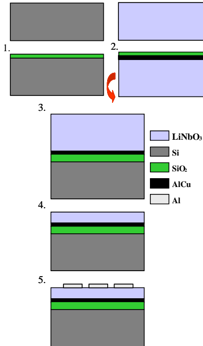
Figure 1. Experimental process for \text{LiNbO}_3 layer transfer technique
