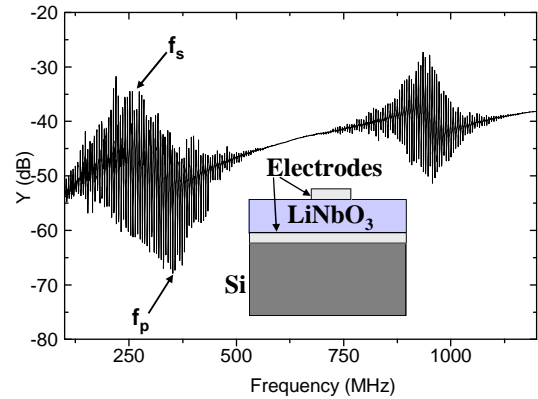
Figure 2. High order harmonics of the HBAR modulated by the first two harmonics of the thinned \text{LiNbO}_3 layer. From the modulation of the thin piezoelectric layer f_s and f_p are the extracted series and parallel resonances of this thin layer. Inset is a schematic view of \text{LiNbO}_3 HBAR.
