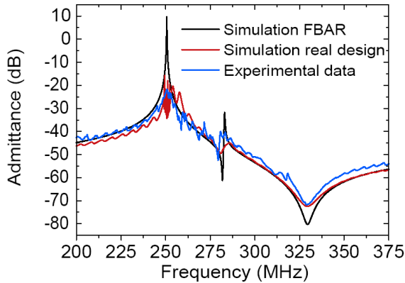
Figure 4. Comparison of the first resonance of a FBAR response simulated considering a homogeneous thickness on the LiNbO 3 (black), assuming an inhomogeneous thickness of the LiNbO 3 plate simulated by 20 resonators connected in parallel (red), and compared to the experimental admittance of the resonator (blue).
