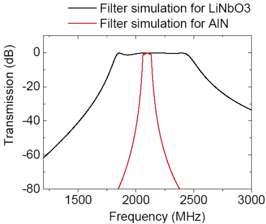
Figure 5. Comparison of non optimized simulated pass band filters based on X-cut LiNbO 3 (black) and traditional sputtered AlN (red). The simulations are performed with the scattering matrix method. The stacks of AlN and LiNbO 3 band pass filters are designed so as to provide centre frequency close to 2 GHz.
