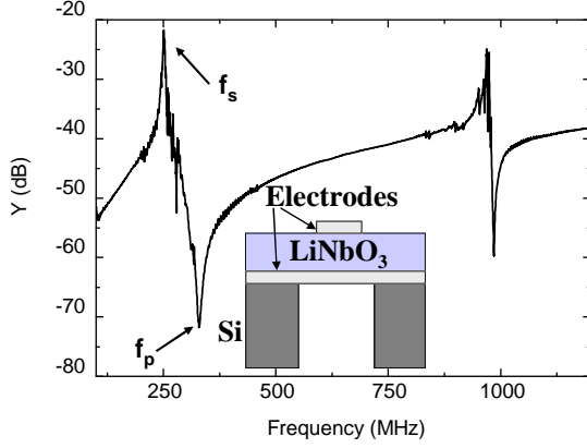
Figure 3. Fundamental and 3 rd harmonics of the pure shear mode of the self-supported thinned X-cut LiNbO 3 plate. A K_t^2 close to 45% is measured. Inset is a schematic view of LiNbO 3 FBAR.
