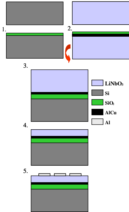
Figure 1. Experimental process for \text{LiNbO}_3 layer transfer technique
