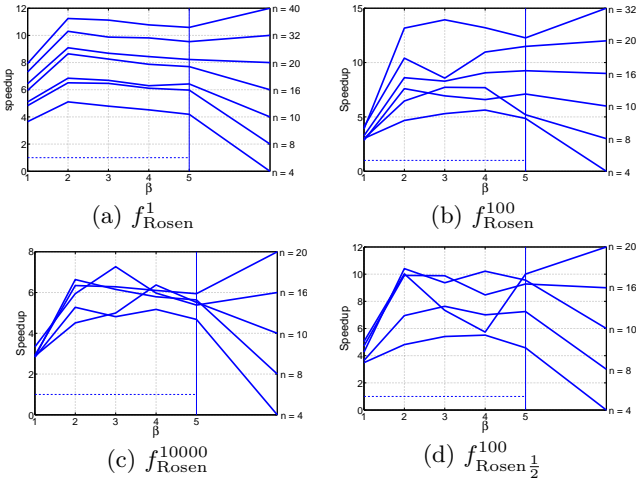
Figure 3: Average speedup with respect to CMA-ES to reach f_{\text{stop}} with a varying number of points used to build the meta-model k_i = \beta \times k_{i,\text{min}} where k_{i,\text{min}} = \frac{n_i(n_i+3)}{2} + 1 . Each point corresponds to 20 runs performed.
