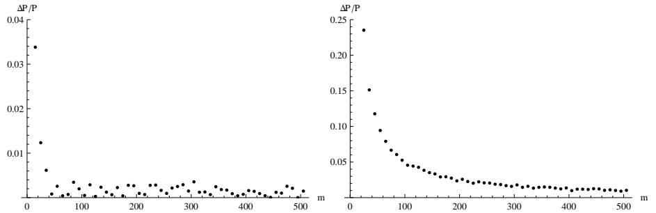
(c) \Delta P/P represents the relative difference between theoretical and measured probabilities. On the left, uniform model with \rho = 0.7 and \nu = 0.3 . On the right, fixed-size model with \rho = 1 , \nu = 0.4 and \mu = 0.6 .
