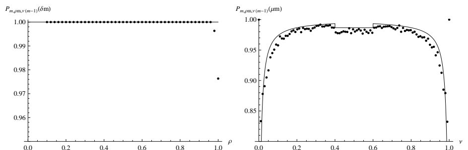
(b) Fixed size uniform model. On the left, m = 100 , \rho varies, \nu = 0.4 , and \mu = 0.5 . On the right, m = 500 , \nu varies, \rho = 1 and \mu = 0.6 .
