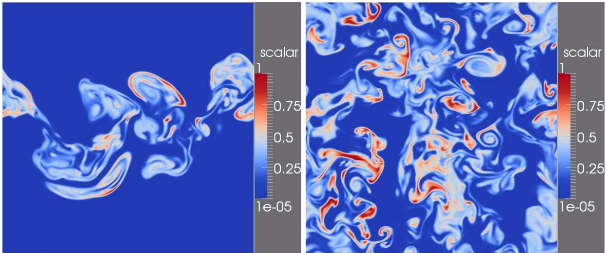
Figure 10: Side and top view of scalar contours at t = 4.5 for the jet (44).
