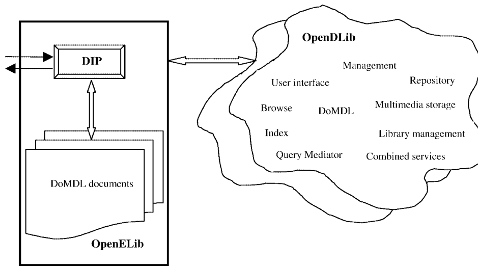
Fig. 3. Interaction OpenELib–OpenDLib.
