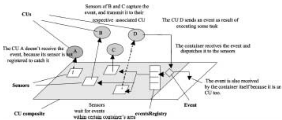
Fig. 1. SAVER architecture.
