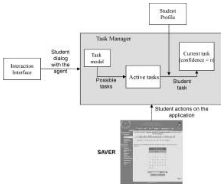
Fig. 4. The Task Manager component.
