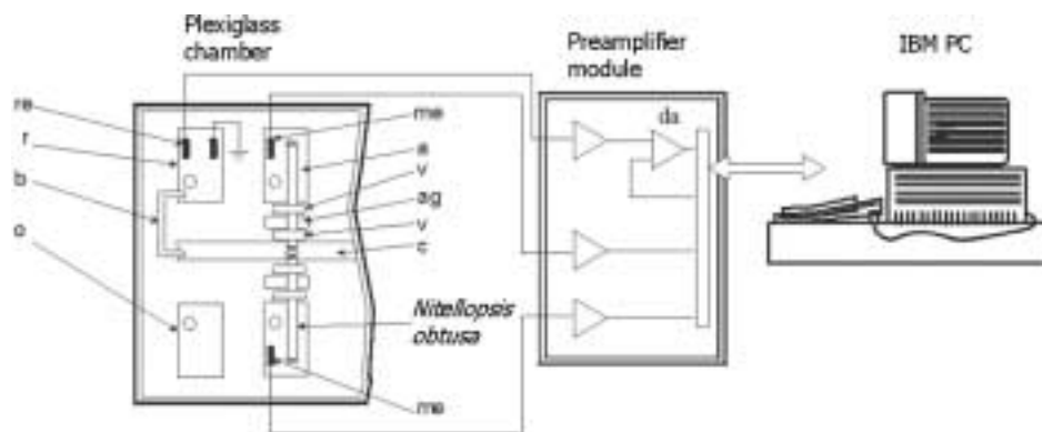
Fig. 4. Schematic diagram of the experimental set-up. See text for details.
