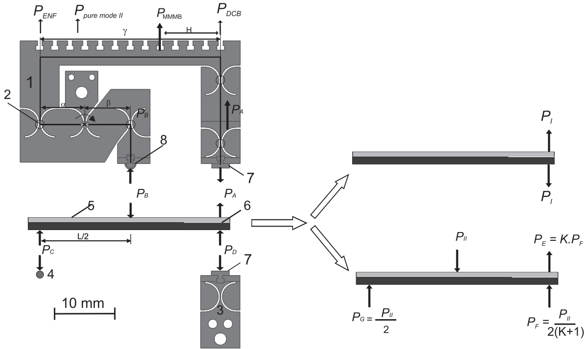
Figure 3. Design of the original MMMB device with: (1) the main loading mechanism (MLM) with (2) elastic hinges, (3) the bottom support hinge, (4) the left support, (5) the bilayer sample with (6) precrack, (7) the dovetail connector, and (8) loading tip. Also shown is the schematic representation of the load distribution under mixed mode bending, with the loads on the sample (shown on the left) and the decomposition of these loads into mode I and pure mode II components (shown on the right).
