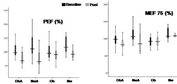
Figure 1. Differences in PEF and MEF 75 obtained at baseline and after 6MWT.
