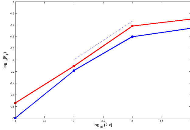
Figure 9: Convergence in space for \mathcal{T}_{\delta x}^1 (red) and \mathcal{T}_{\delta x}^2 (blue). Dotted line has slope 2/3.
